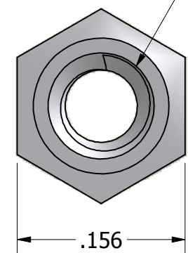
2-56 UNC-2B Thru
