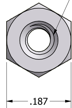
2-56 UNC-2B Thru
